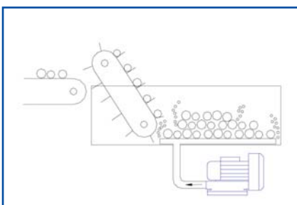
Secado de frutas Vegetable & Fruit Washer
