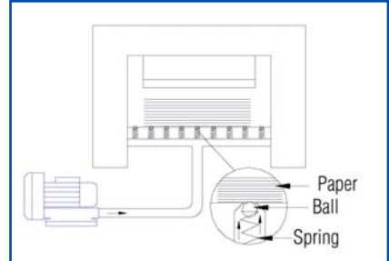
Artes Gráficas Floating Element of Paper Cutter
